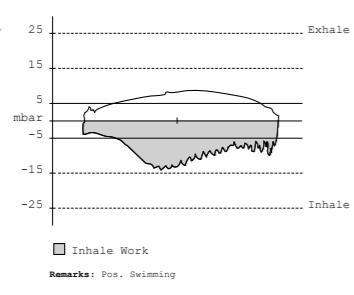
Pressure-Volume Diagrams at Mean Depth of 50.5 msw (165.8 fsw)
