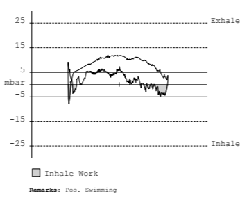
Pressure-Volume Diagrams at Mean Depth of 50.2 msw (164.8 fsw)
