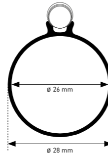
BARREL SECTION
